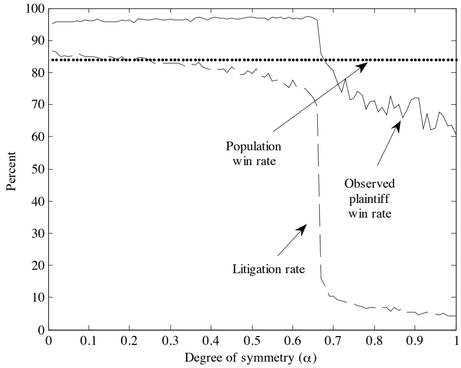
Figure 1: Priest and Klein simulation results
